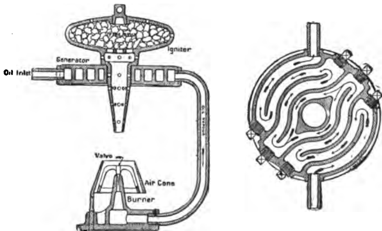
FIG. 206.—The "House" Kerosene Vapor Burner, section in elevation, and plan section of the vaporizing chamber, or "generator," showing course of oil in process of being converted into vapor under heat of the flame.
